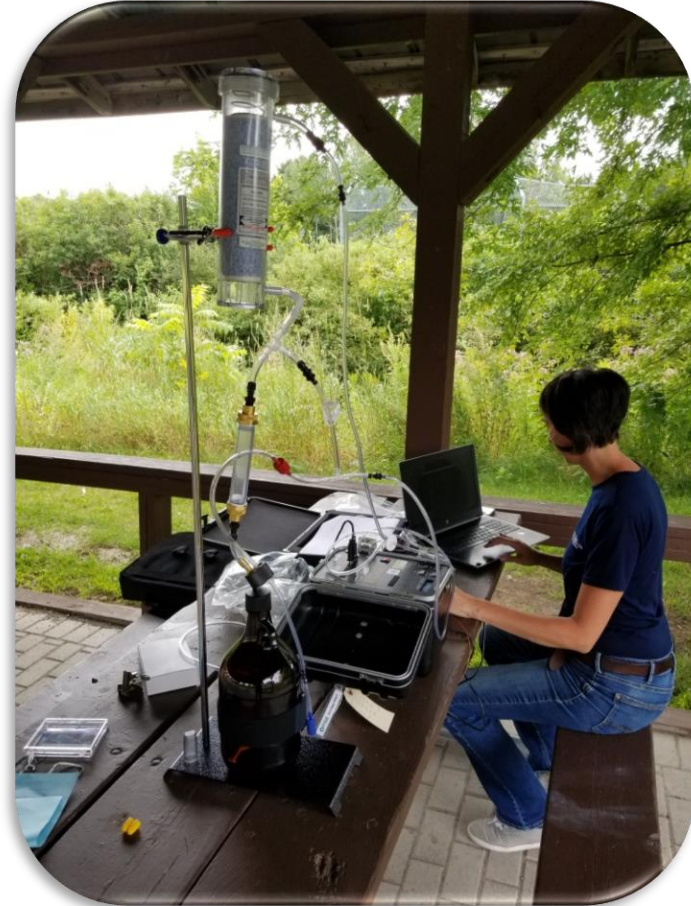
Sampling water for radon gas Shields Creek, Greely
